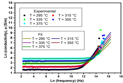
Fig 6: the plot of \ln(\sigma f) versus \ln(f) at different temperatures for \text{Mo}_6\text{SnS}_8 thin film
