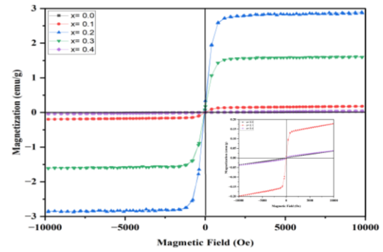
Fig. 5: Magnetization versus magnetic field for \text{BiFe}_{1-x}\text{Y}_x\text{O}_3 ceramics ( x = 0.0-0.4 ) at room temperature. Inset: enlarged M-H loops for x = 0.0, 0.1 , and 0.4
