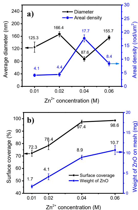
Fig. 3: a) Diameter and areal density; b) Average surface coverage and weight of ZnO NRs on Kanthal mesh. Data was measured from FESEM images of Fig. 2
