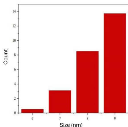
Fig. 4: Zetasizer count
