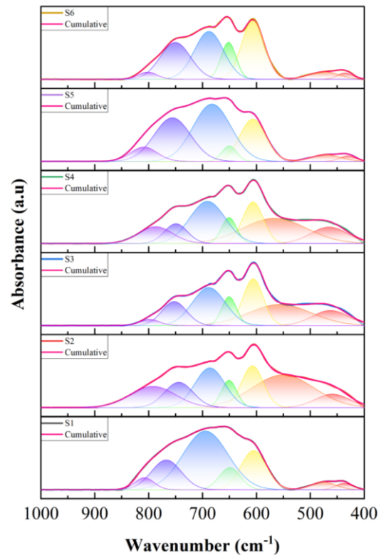
Fig. 3: The deconvolution of FTIR spectra in the region 400 – 1000 \text{cm}^{-1} for all samples.
